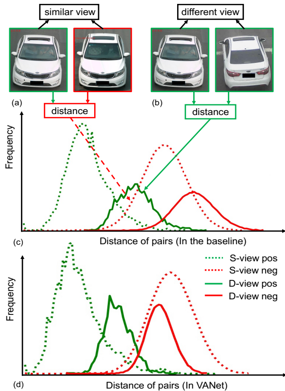
Figure 1. Illustration of vehicle re-ID with viewpoint variations. Two different vehicles from similar viewpoints (a) appear more similar than the same vehicle observed from different viewpoints (b). (c) distance distribution of a baseline method (see Tab. 1). (d) distance distribution of proposed VANet method. S-view pos: positive pairs from S-views. S-view neg: negative pairs from S-views. D-view pos: positive pairs from D-views. D-view neg: negative pairs from D-views. In the baseline (c), the “D-view pos” are not well separated from “S-view neg”. In VANet (d), the distances of “D-view pos” become smaller, while the distances of “S-view neg” become larger. They are better separated.
